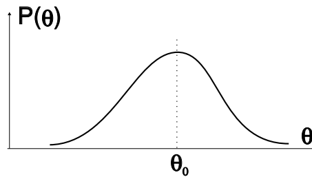
Normal distribution
