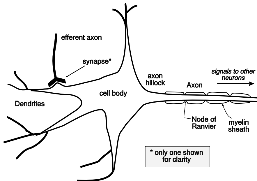
Biological neuron
